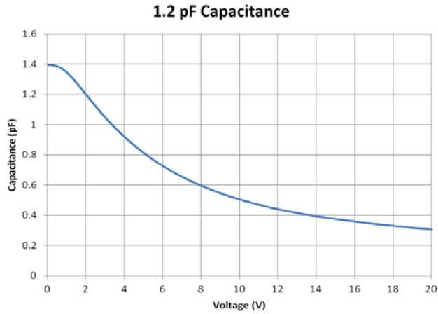
Figure 1. Capacitance
