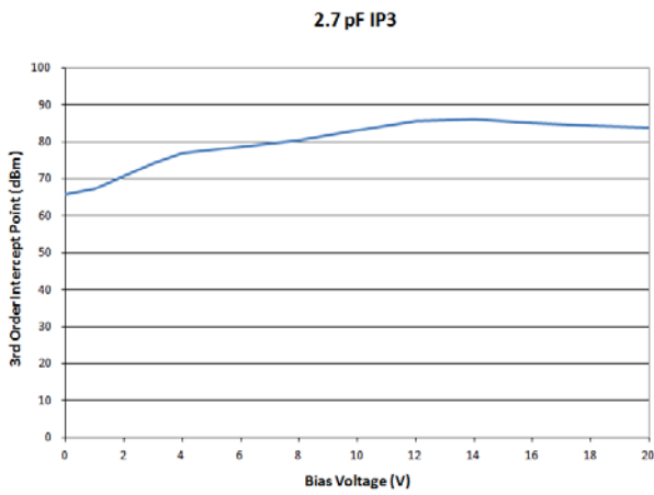
Figure 3. IP3*
